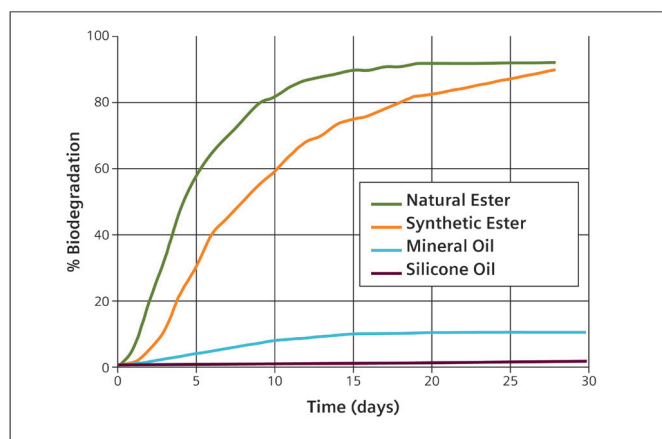
Figure 4. Comparison of biodegradability of insulation fluids [7]
