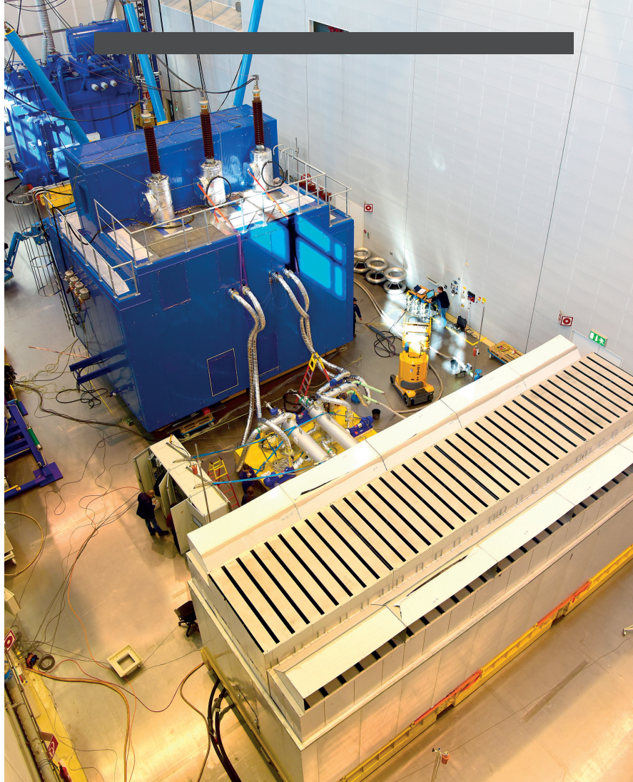
Figure 6. Transformer cooling system (heat exchanger) special silencers in the test bay
