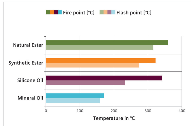
Figure 2. Comparison of the fire and flash points of various insulation oils [1]
