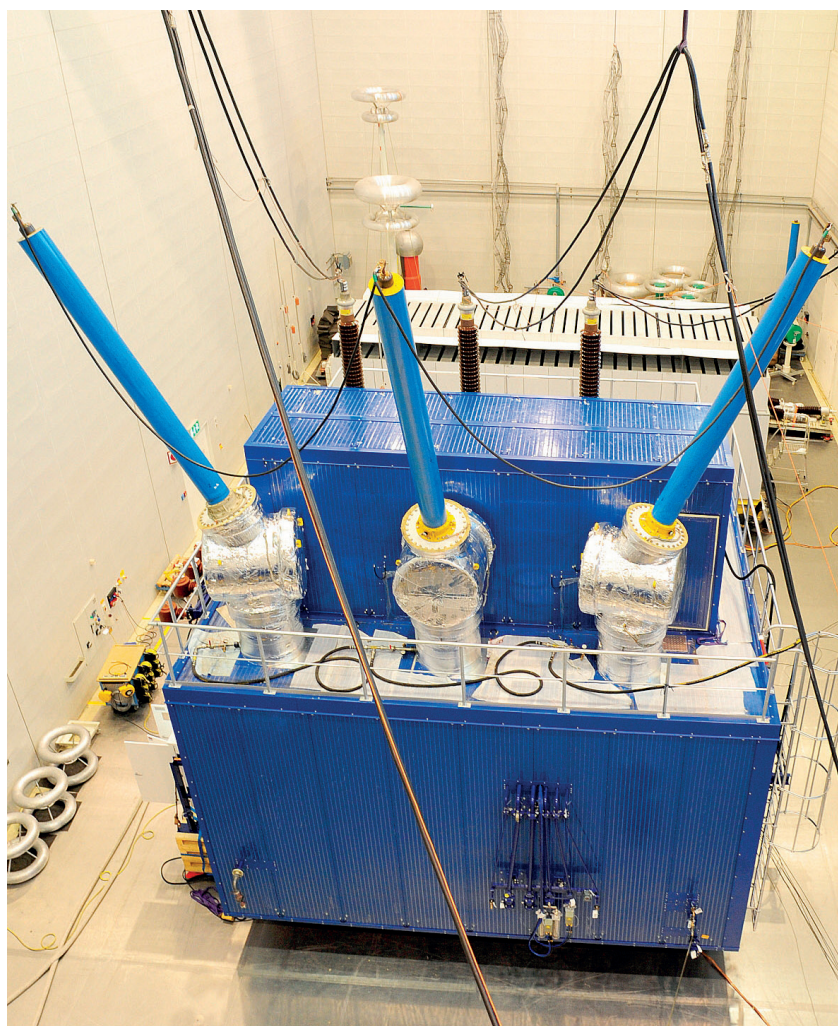
Figure 5. Transformer with thermal insulation (enclosure) in the test bay
