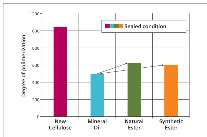
Figure 3. Results of polymerization aging test in various insulation liquids [1]
